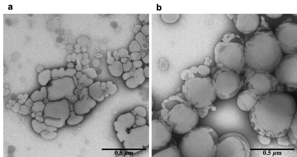
Fig. 6 Representative transmission electron micrographs of PL-90 g liposomes without (a) and with (b) encapsulated OLE
