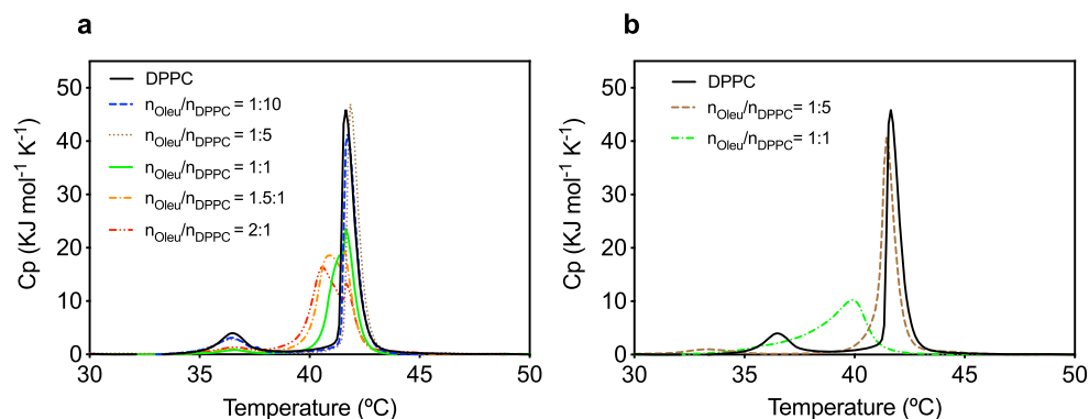
Fig. 1 Differential scanning calorimetry thermograms (as measures of C_p : specific heat) of 1,2-dipalmitoyl-sn-glycero-3-phosphocoline (DPPC) liposomes with passively (a) and actively (b) encapsulated oleuropein at different oleuropein:DPPC molar ratios (as indicated), in 20 mM HEPES (pH 7.0)
