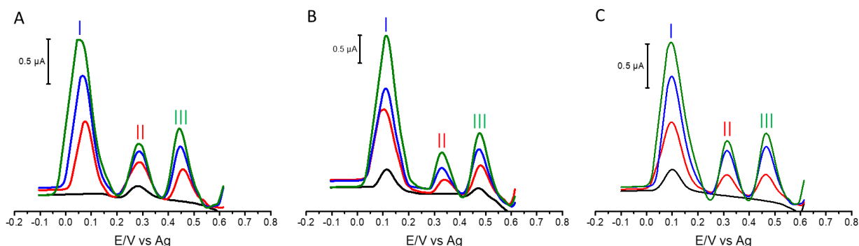
Fig. 5 Differential pulse voltammograms for sample analysis at SPE-CB-WS 2 /AuNP-CT sensor. Class-selective hCNs-based determination in food samples: rapeseed oil extract (A), kalanchoe Crenata (B) and apple juices (C); Peak I (CF equivalents), Peak II (SP equivalents), Peak III (CM equivalents). Samples spiked with three increasing concentrations of the mixture of CF, SP, and CM (unspiked samples: black line). Spiked samples, CF, SP, and CM concentration, respectively: 5, 10, and 15 \mu\text{mol L}^{-1} (red line); 10, 20, and 30 \mu\text{mol L}^{-1} (blue line); 15, 30 and 45 \mu\text{mol L}^{-1} (green line). Conditions: 0.1 \text{mmol L}^{-1} PB + 0.1 KCl, pH 7.0; pulse width 50 ms, modulation amplitude 50 mV, scan rate of 25 \text{mV s}^{-1} .
