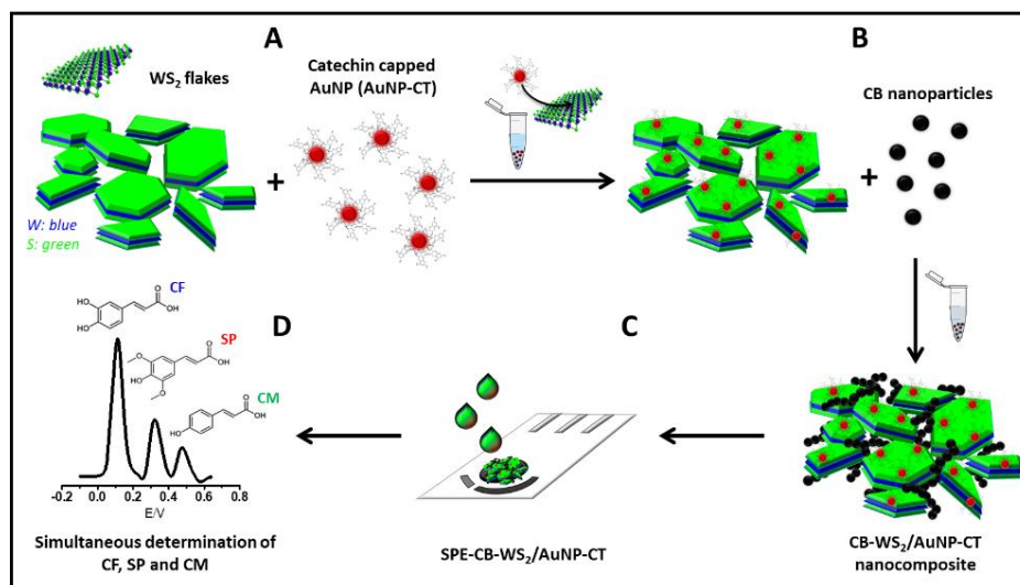
Scheme 1. Scheme of the SPE-CB-WS 2 /AuNP-CT architecture for hydroxycinnamic acid structural analogs electrochemical sensing. A: WS 2 decoration with AuNP-CT (a detailed scheme of this step is depicted in Scheme S1); B: assembly of WS 2 /AuNP-CT into CB. C: SPE modification with the CB-WS 2 /AuNP-CT nanocomposite. D: DPV simultaneous determination of CF, SP, and CM.
