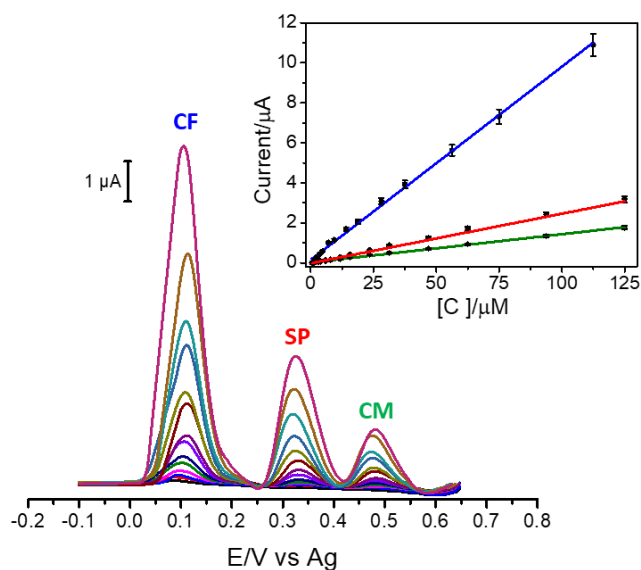
Fig. 4 Differential pulse voltammograms for the simultaneous calibration of CF (0.3-112.0 μmol L -1 ), SP (1.2-125.0 μmol L -1 ), and CM (1.3-125.0 μmol L -1 ) at SPE-CB-WS 2 /AuNP-CT sensor. Insets: calibration plots for CF (blue line), SP (red line), and CM (green line) (n=15 assayed concentrations, n=3 replicates each). Conditions: 0.1 mmol L -1 PB + 0.1 KCl, pH 7.0; pulse width 50 ms, modulation amplitude 50 mV, scan rate of 25 mV s -1 .
