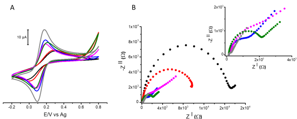
Fig. 2 Electrochemical characterization of the set of electrodes: (A) cyclic voltammograms at 50 mV s -1 and (B) electrochemical impedance spectra (inset reports the Nyquist plot magnification at low frequencies region). Conditions: 1 mmol L -1 [Fe(CN) 6 ] 3-/4- redox probe in 0.1 mol L -1 KCl (pH 7.0). The code colour-based legend is as follows bare SPE (black), SPE-WS 2 (red), SPE-CB (blue), SPE-WS 2 /AuNP-CT (violet), SPE-CB-WS 2 (green), and SPE-CB-WS 2 /AuNP-CT (grey).
